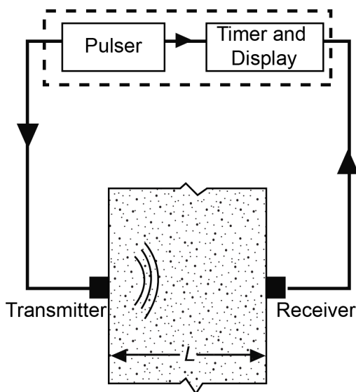
Figure 1-3: Ultrasonic pulse velocity test [3]
