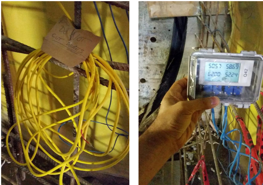
Figure 3-3: Drawbacks of wired systems
