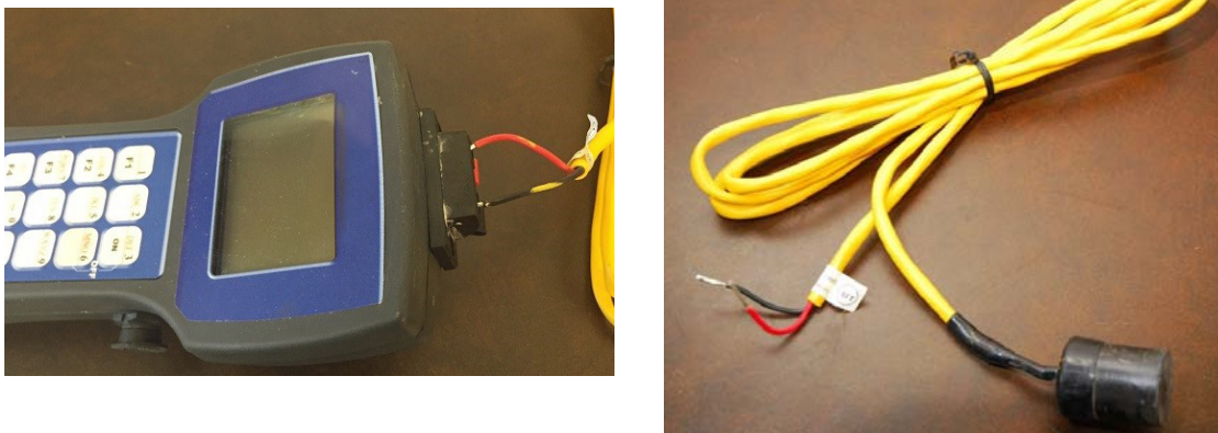
Figure 3-2: Wired system
