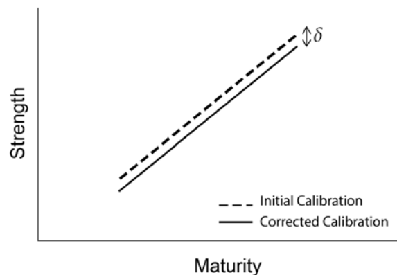
Figure 5-7: Maturity calibration including safety factor
