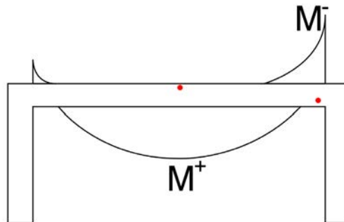
Figure 6-3: Compression locations for positive and negative moments.
