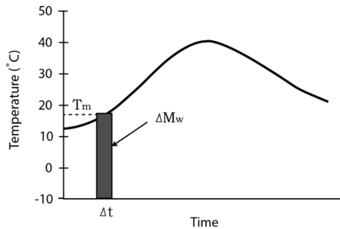
Figure 4-5: Weighted maturity [30]
