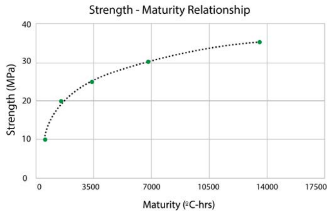
Figure 5-6: Example-Maturity-strength relationship
