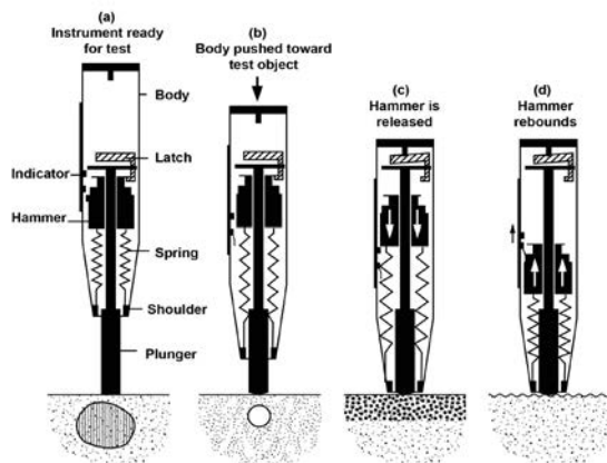
Figure 1-1: Rebound hammer test [3]
