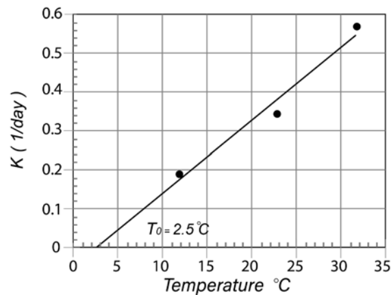
Figure 4-4: Datum temperature
