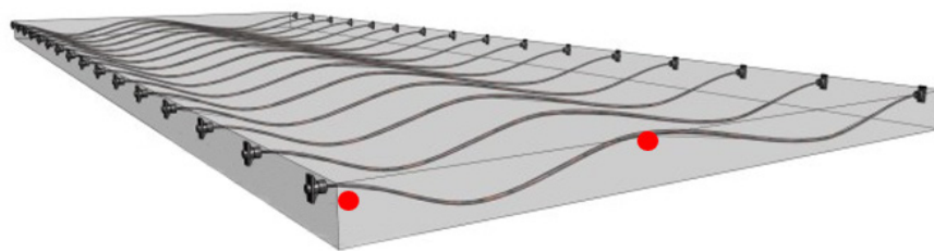
Figure 6-5: Location of maturity monitoring in post tensioning element [41]
