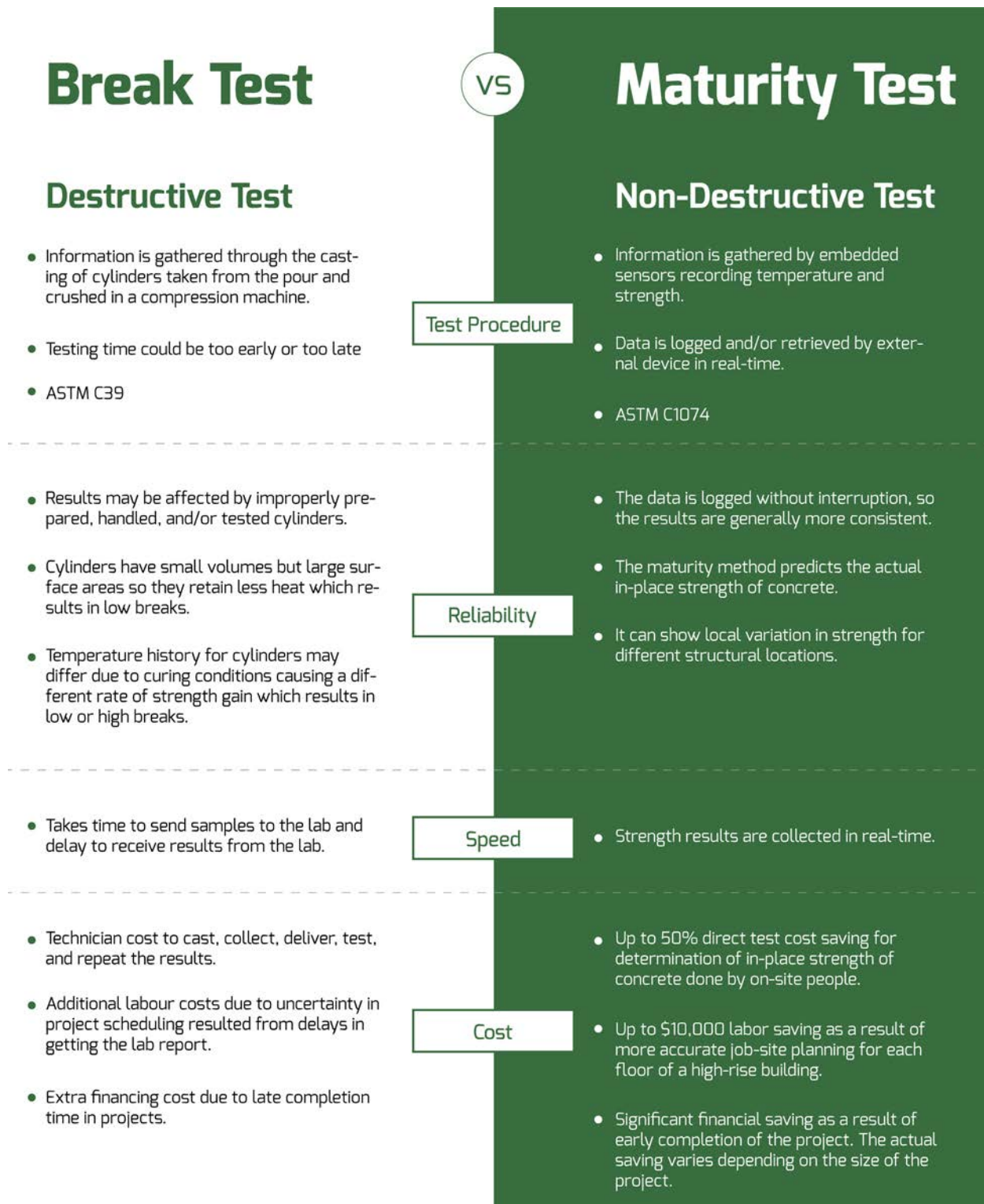
Figure 2-3: Break test vs. Maturity test
