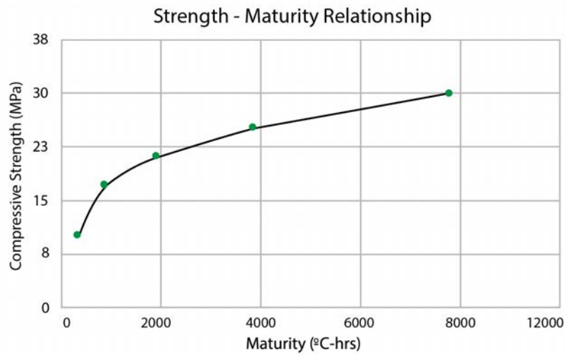
Figure 2-2: Example of a maturity-strength relationship
