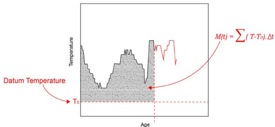
Figure 4-1: Temperature-Time Factor method
