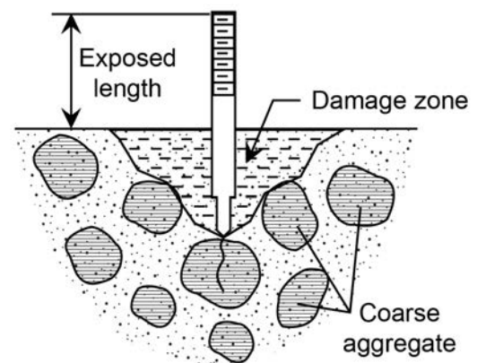
Figure 1-2: Penetration resistance test [3]
