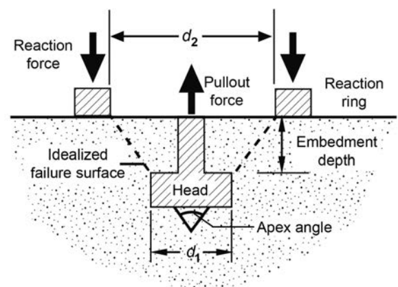
Figure 1-4: Pullout test [3]
