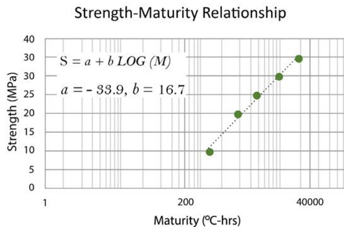
Figure 5-1: Example of strength-maturity relationship equation
